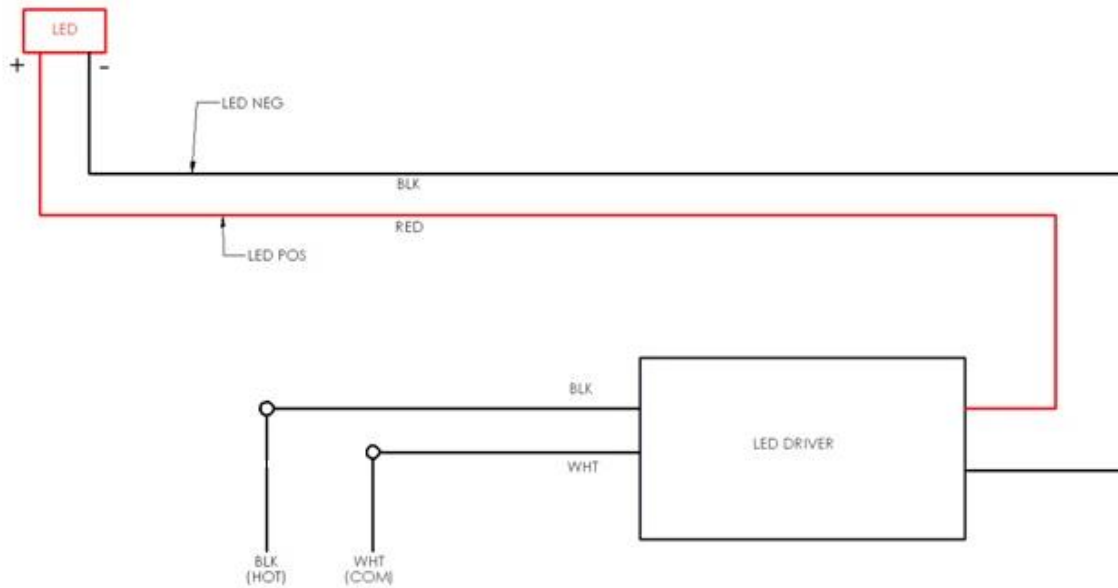
WIRING DIAGRAM
