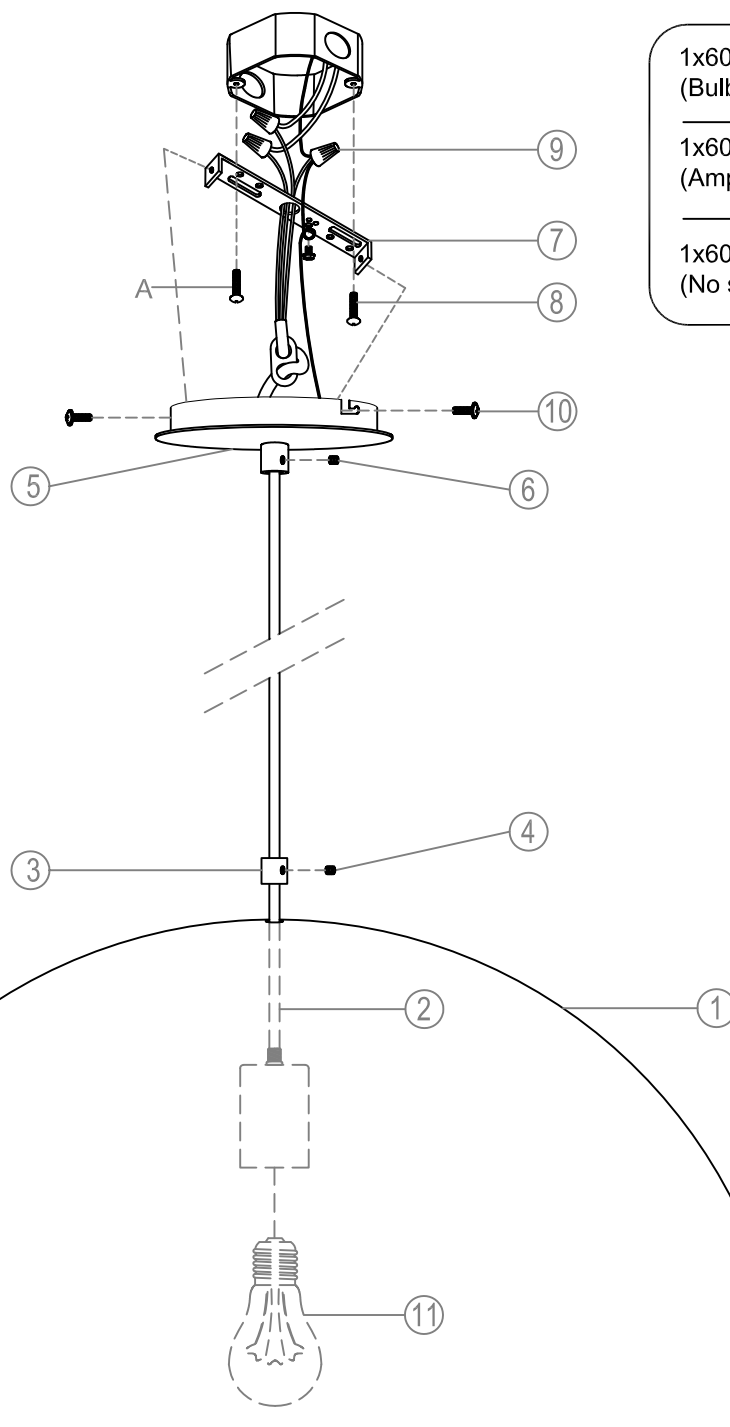
Wire connection
